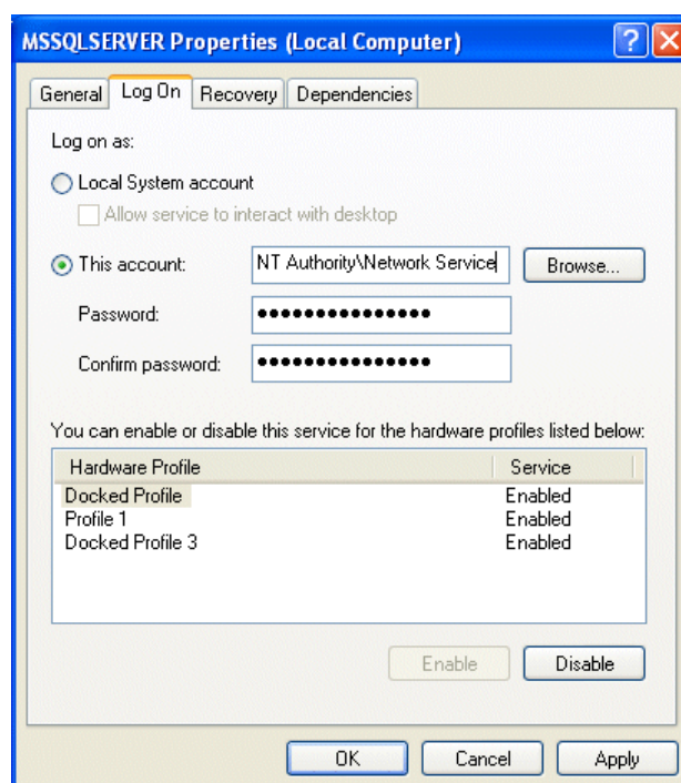
SQL Server Service Properties window
